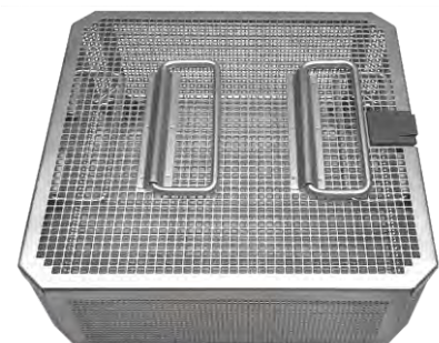
7-120-01 Instrument Tray for 3.0mm Cannulated Cancellous Screw Instrument Set
